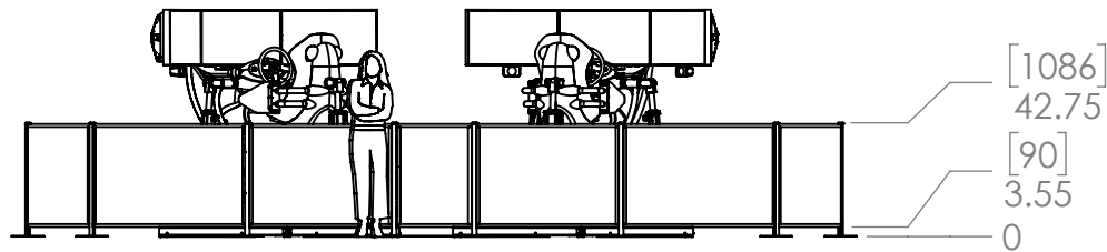
Side Elevation
