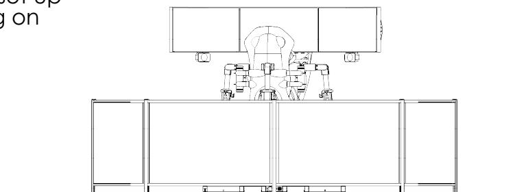
Back Elevation
